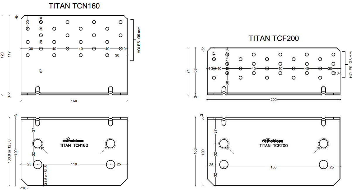
Figure B. 9 Dimensions of Angle Bracket TITAN TCN160
