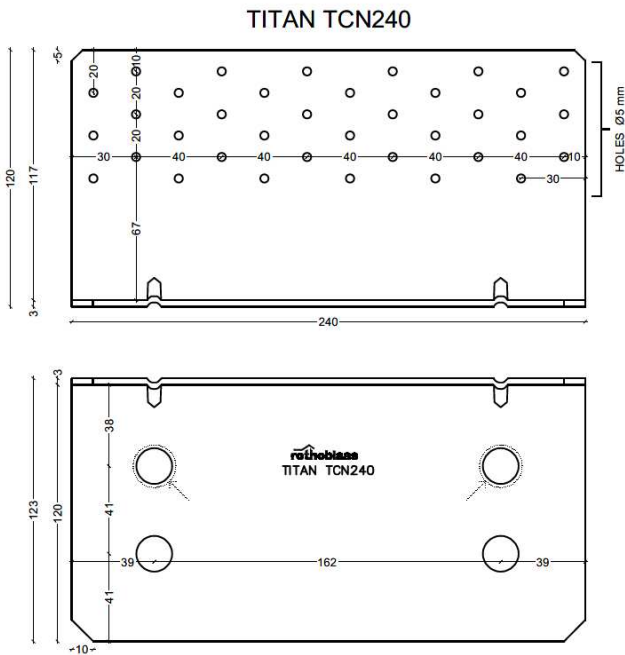
Figure B. 12 Dimensions of Angle Bracket TITAN TCN240
