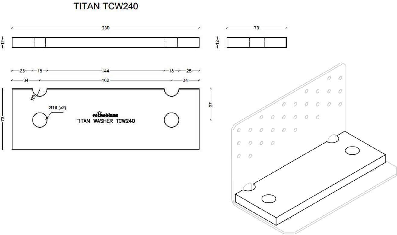
Figure B. 17 Dimensions of TITAN Washer TCW240
