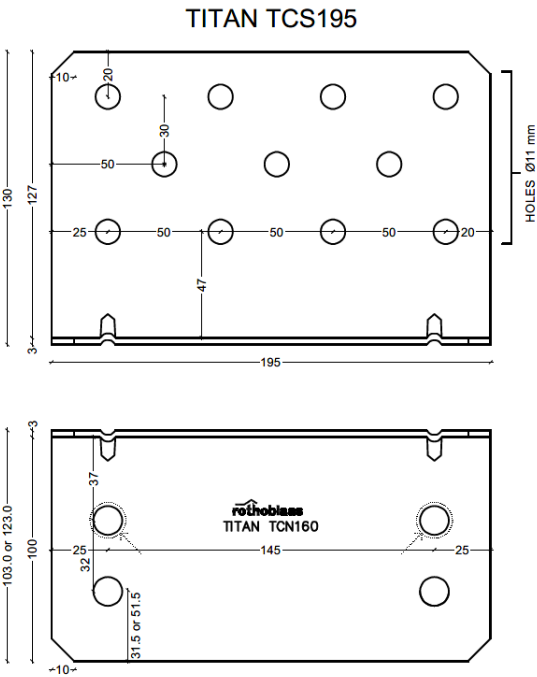
Figure B. 14 Dimensions of Angle Bracket TITAN TCS195
