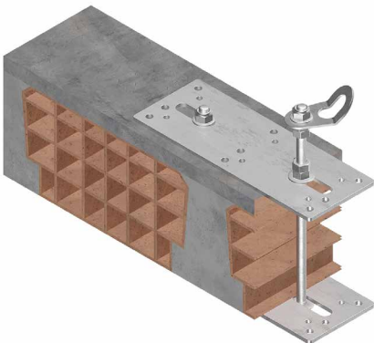
MULTIPLATE+MULTIPLATE
