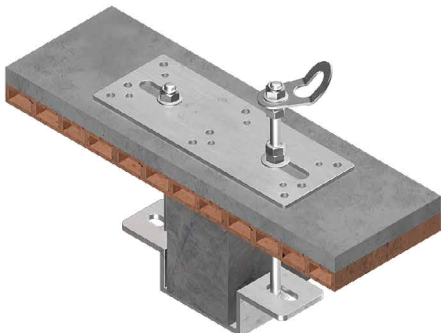
MULTIPLATE+OMEGA
